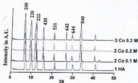
Figure 1. X-ray diffraction patterns of H-A/Co-A zeolite.
